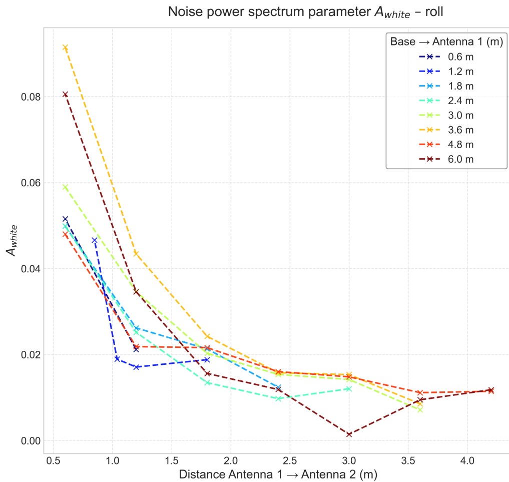
Figure 1.18: Amplitude of the white noise amplitude for the roll data as a function of the distance between the antennas, for different distances between the base and antenna 1.
