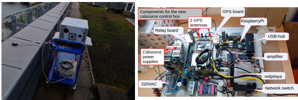
Figure 1.3: (left) Photo of the calibration box, on top of the chariot. (right) Photo of the inside of the calibration box. The GPS PCB is included within the box. The integration was made by Claude Boutonnet at APC.
