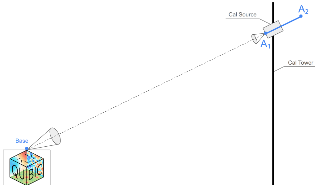
Figure 1.20: Drawing to show the expected position for the GPS antennas. The base antenna is located as close as possible from QUBIC line-of-sight, on the left. On the right, the Calibration Source is fixed on the Calibration Tower, the Antenna 1 (A1) is attached as close as possible from the line-of-sight of the source, while the Antenna 2 (A2) is placed on a rigid rod, again align with the line-of-sight.
