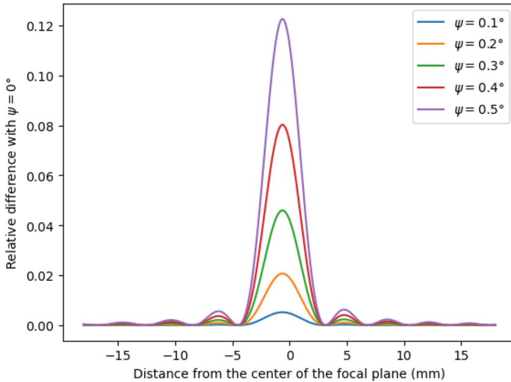
Figure 1.6: Plot showing the beam relative difference in amplitude between the case where the calibration source is aligned with QUBIC's line of sight and when the source is rotated by an angle \psi around the vertical axis. It shows that the more the source is deviated from the line of sight, the lower the beam amplitude becomes, emphasizing the need to track calibration source position and orientation. The plot is build from simulation data made by Sabrina Marwede from Maynooth University, a PhD Student working on optical simulation for QUBIC.
