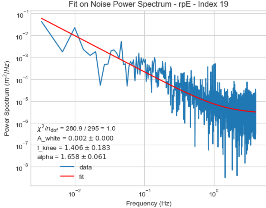
Figure 1.16: Power Spectrum (in blue) for rpE data for the configuration 19. The fitted model 1.3 is displayed (in red) above the data. The parameters value of the model and their associated error is shown, in addition to the \chi^2 value divided by the degree of freedom.
